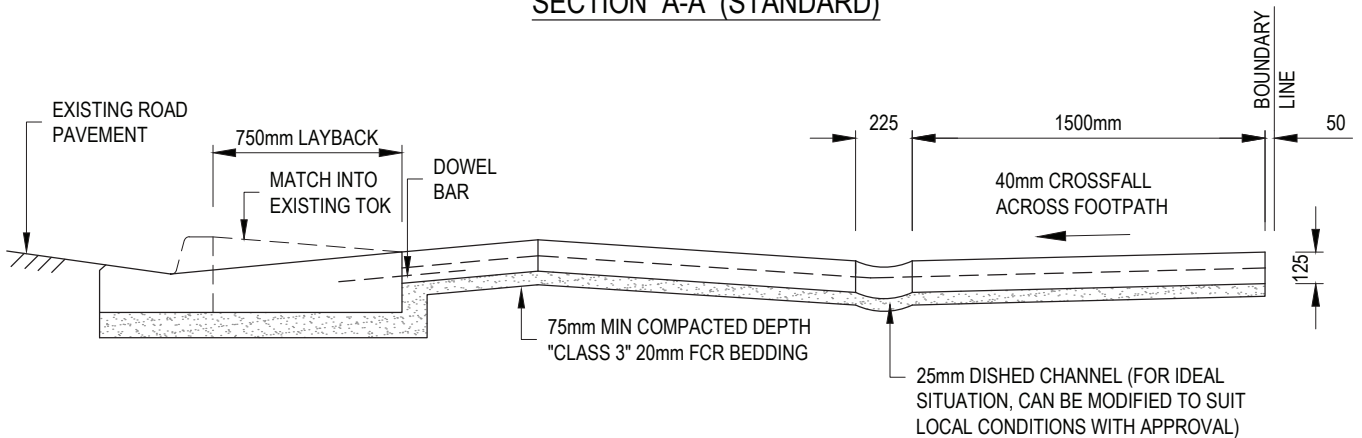
SECTION A-A (REVERSE FALL) (ONLY TO BE USED WITH COUNCIL APPROVAL)
