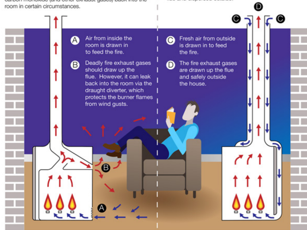
Diagram from Energy Safe Victoria. 2024. Open-flued gas space heaters FAQ.
